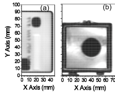
Fig. 2: Terahertz image of (a) Visa card (b) plastic box with a mirror inside at 0.292THz.
